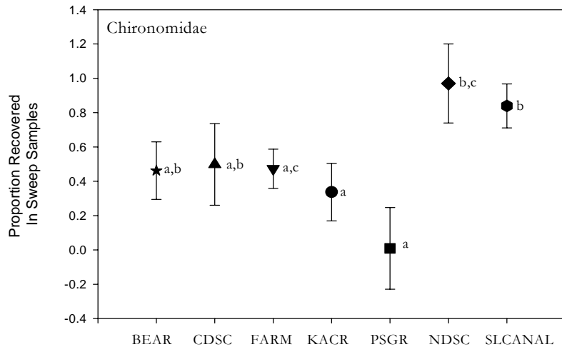
Figure 9. Mean proportion ( \pm SE) of chironomidae recovered from sweep samples at each site. Means with the same letter are not significantly different ( P < 0.05 ).
